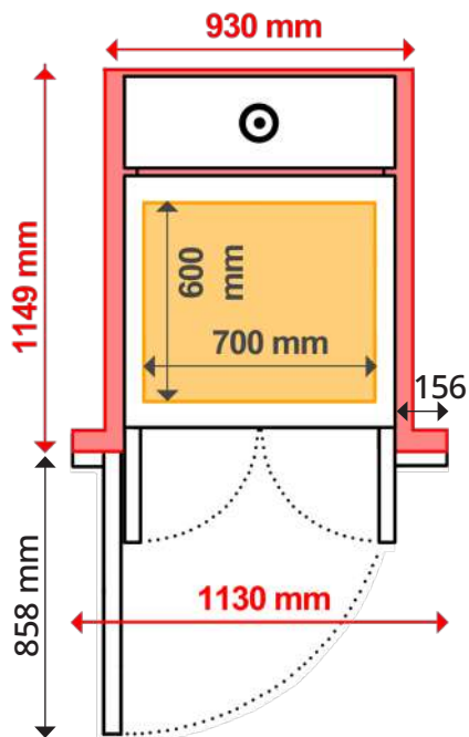
S Size TOP FLOOR - GATE
