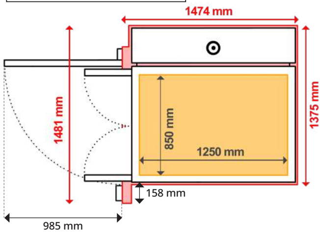
XL Size TOP FLOOR - GATE
