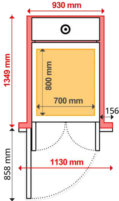
M Size TOP FLOOR - GATE
