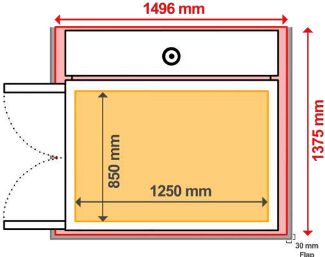
XL Size TOP FLOOR - HATCH
