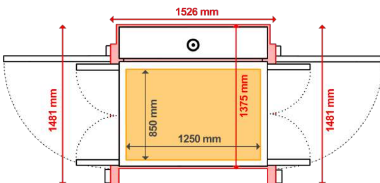
XL Size TOP FLOOR - DOUBLE GATE
