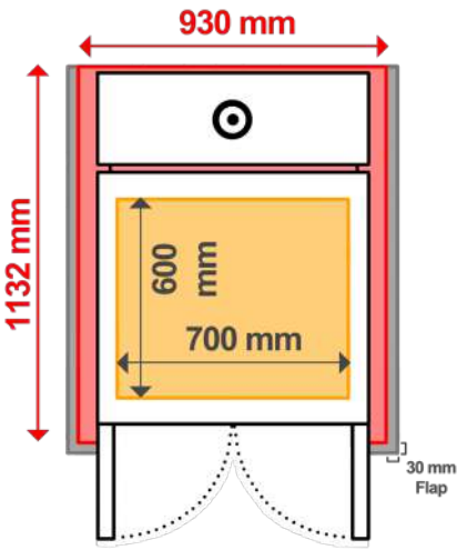
S Size TOP FLOOR - HATCH
