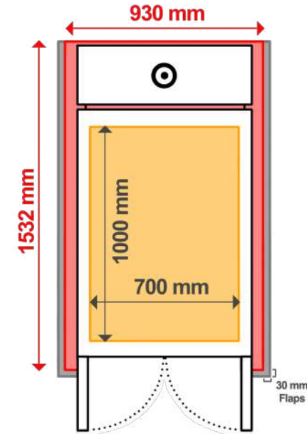
L Size TOP FLOOR - HATCH
