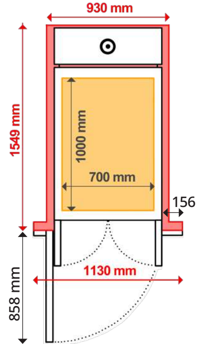
L Size TOP FLOOR - GATE
